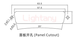
面板开孔 (Panel Cutout)
