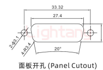
面板开孔 (Panel Cutout)
